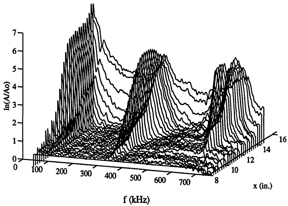
Figure 5.9 Disturbance Spectra in the Cooled-Cone Boundary Layer (Oblique View)
