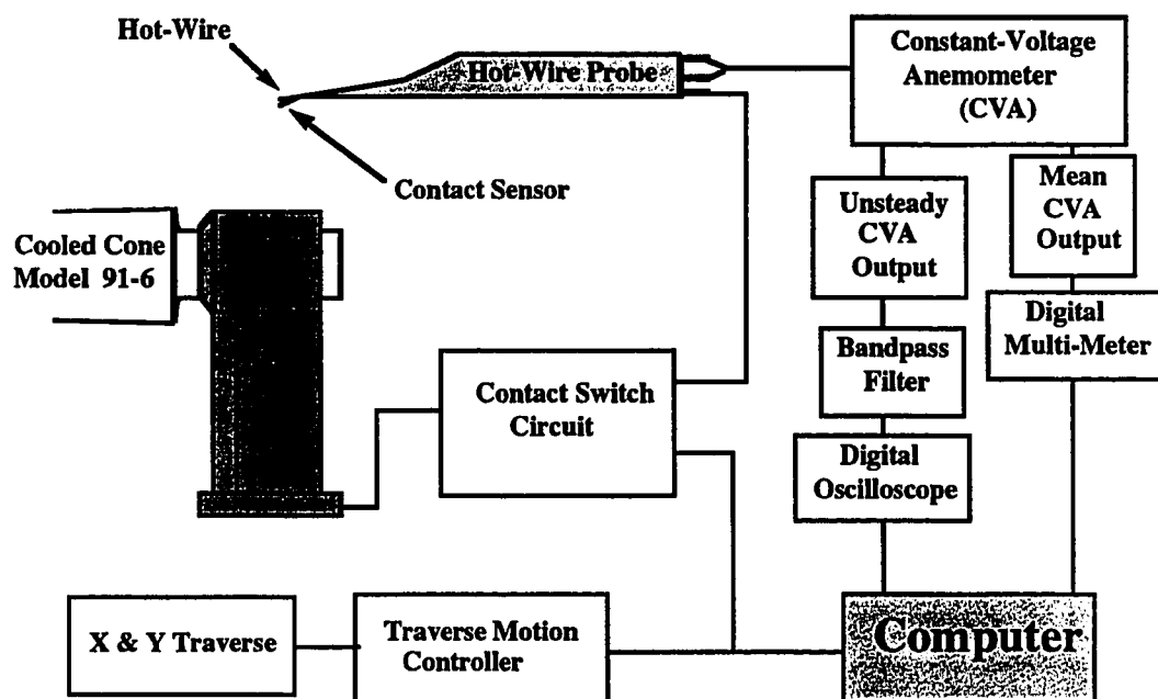
Figure 2.11 Schematic of Data Acquisition System
