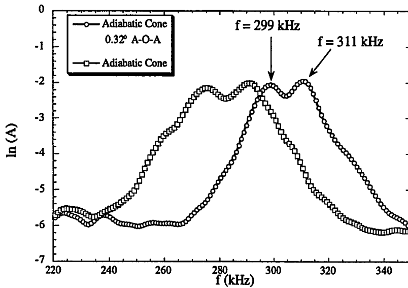
Figure 6.10 Variation in Wave-Packet Frequencies with 0.32^\circ A-O-A (Windward Side Measurements, x=14.25 in.)
