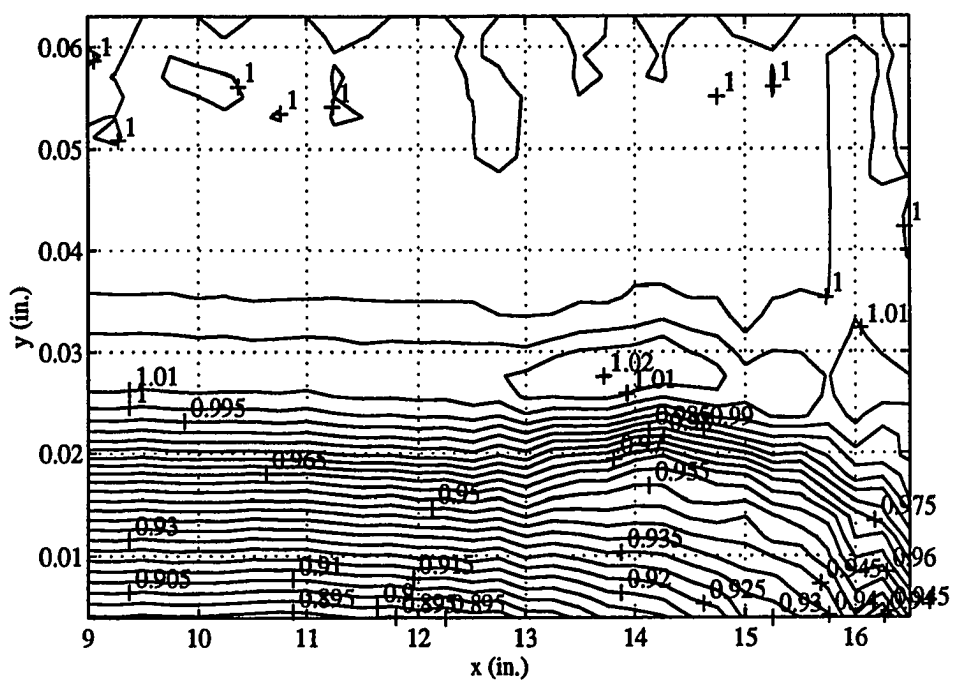
Figure 5.3 Contour Plot of Normalized R_w (Cooled Cone)
