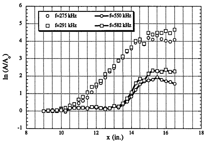
Figure 4.14 Growth of Second-Mode Disturbances and Harmonics (Adiabatic Cone)
