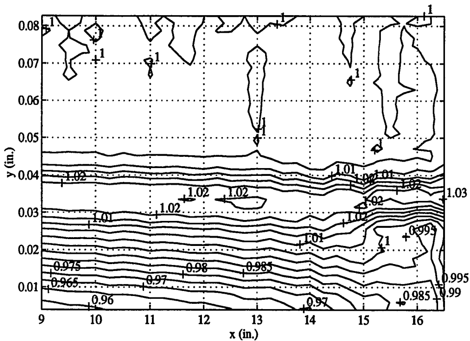
Figure 6.9 Contour Plot of Normalized R_w in the Adiabatic-Cone Boundary Layer with 0.32^\circ A-O-A (Windward Side Measurements)
