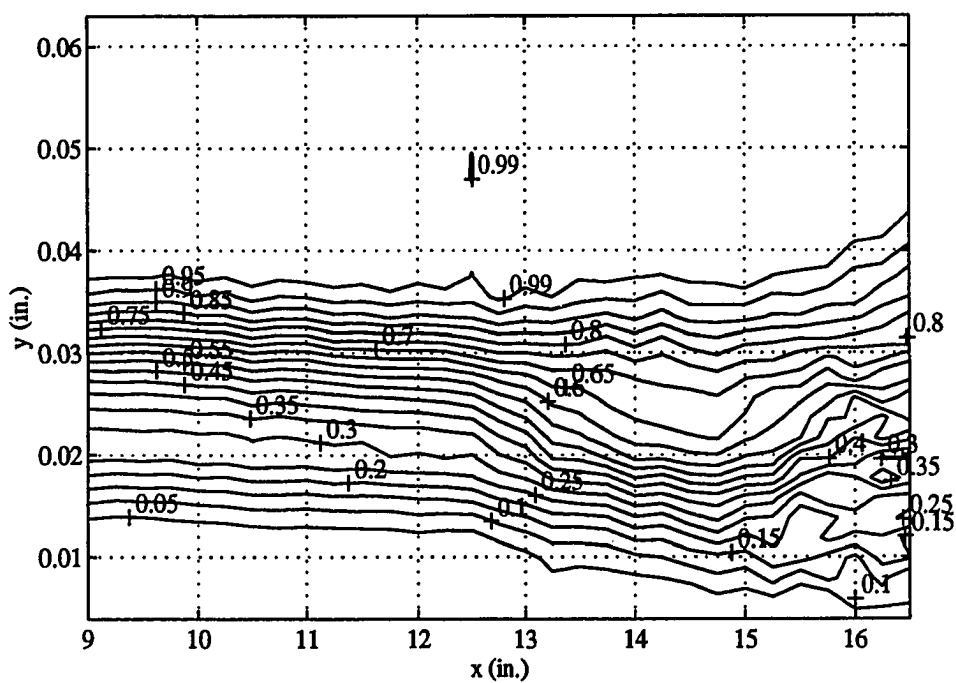
Figure 5.4 Contour Plot of Normalized V_{s,mean} (Cooled Cone)
