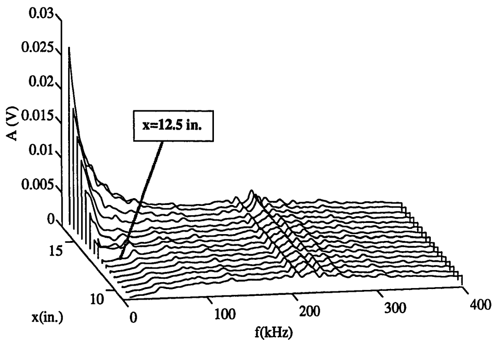
Figure 3.2 Freestream Spectra at y = 0.24 in.
