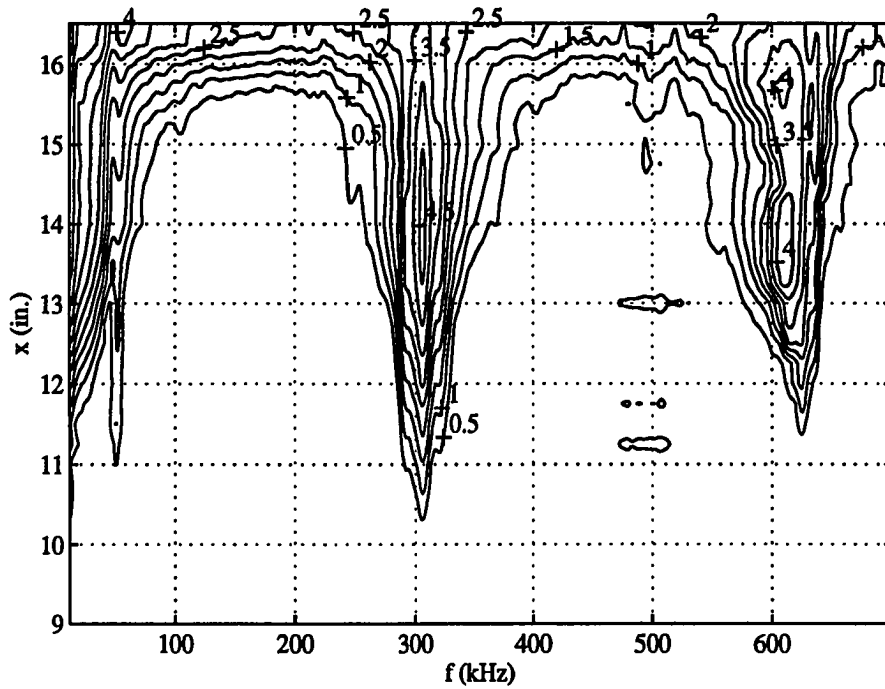
Figure 5.11 Disturbance Spectra in the Cooled-Cone Boundary Layer (contour plot)
