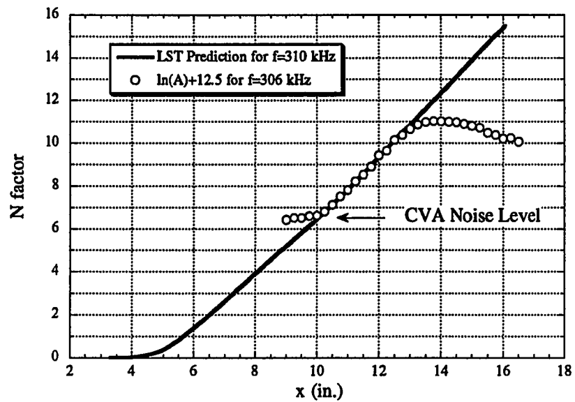
Figure 5.13 Disturbance Growth Chart for the Cooled-Cone Boundary Layer
