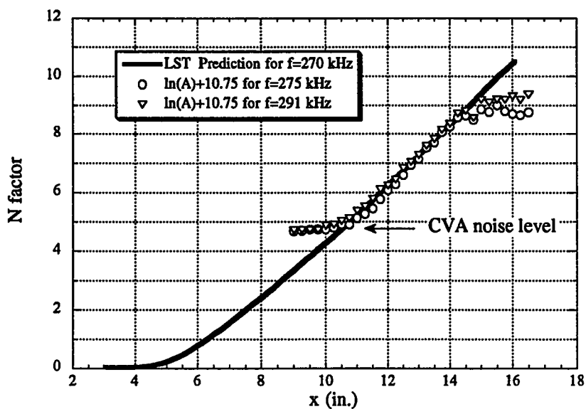
Figure 4.13 Disturbance Growth Chart for the Adiabatic-Cone Boundary Layer
