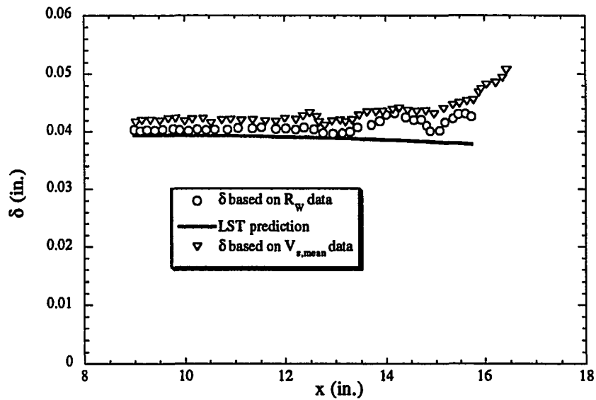
Figure 5.5 Boundary-Layer Thickness (Cooled Cone)
