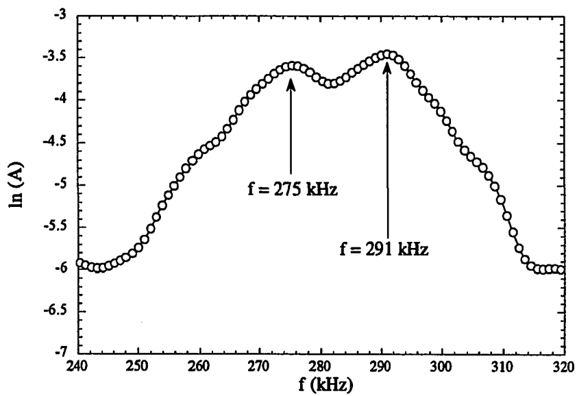
Figure 4.12 Second-Mode Disturbance Band (Adiabatic Cone, x=13 in.)
