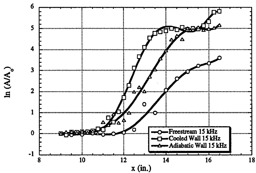
Figure 7.6 The Growth of Disturbances at 15kHz
