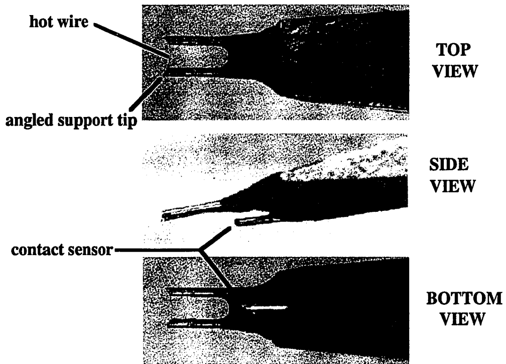
Figure 2.4 Custom Hot-Wire Probes
