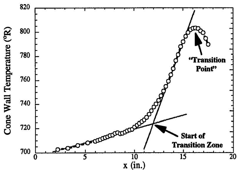
Figure 4.1 Wall Temperature (Adiabatic Cone)
