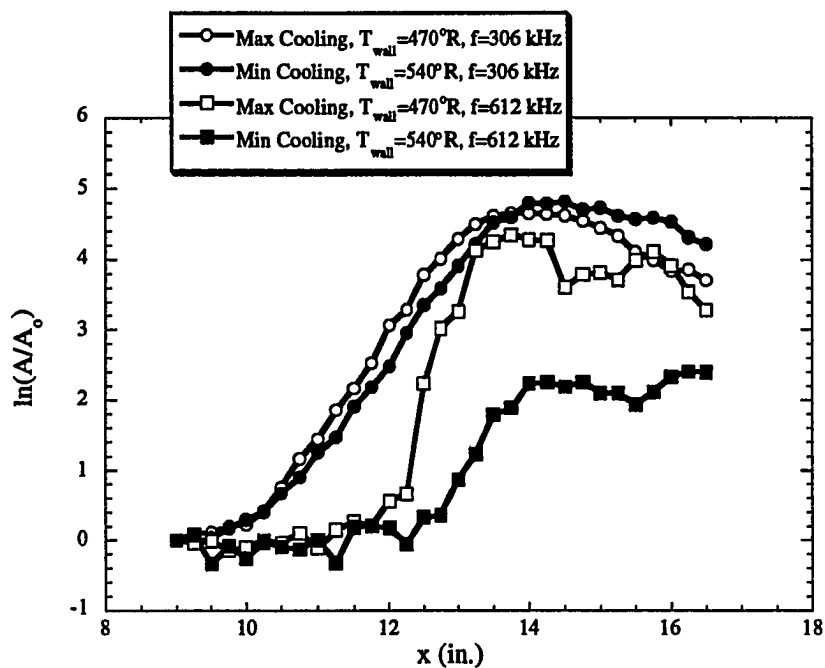
Figure 6.5 Variation in Disturbance Growth with Cooling Rates
