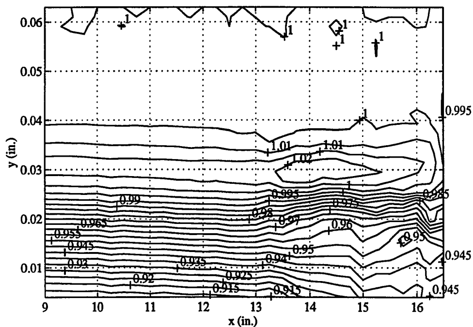
Figure 6.3 Contour Plot of Normalized R_w with Minimal Cooling
