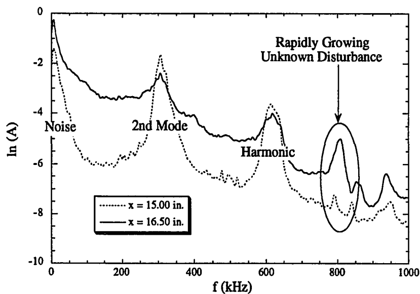
Figure 5.18 Spectral Growth in the Nonlinear Region (Cooled Cone)
