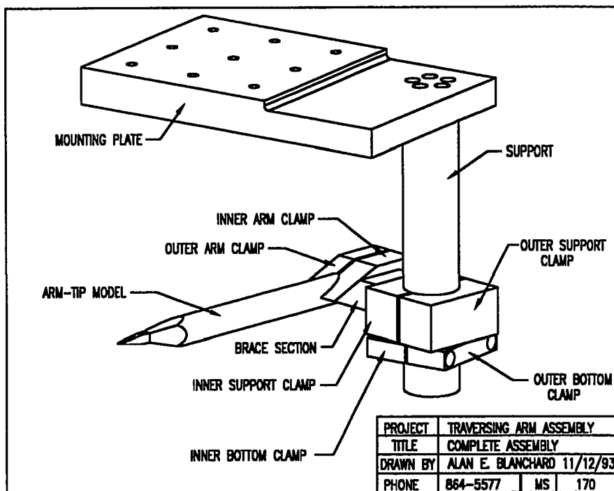
Figure 2.8 Traversing Arm
