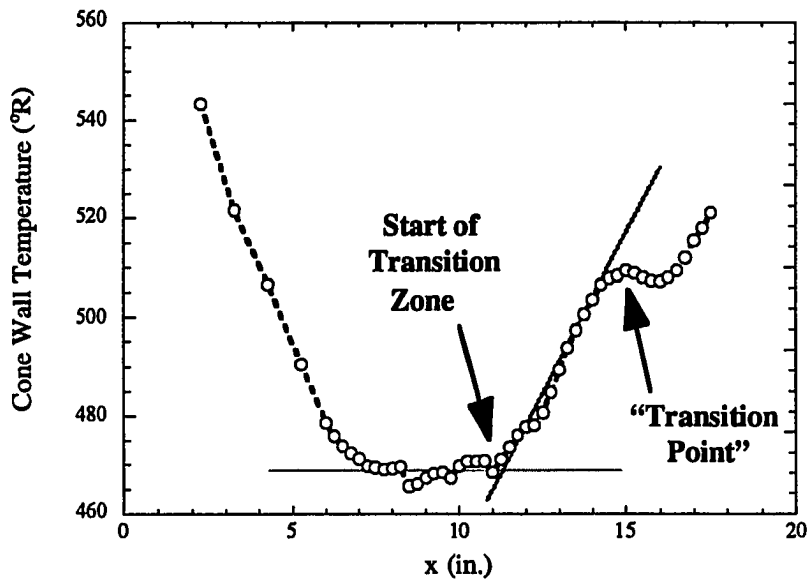
Figure 5.1 Wall Temperature (Cooled Cone)
