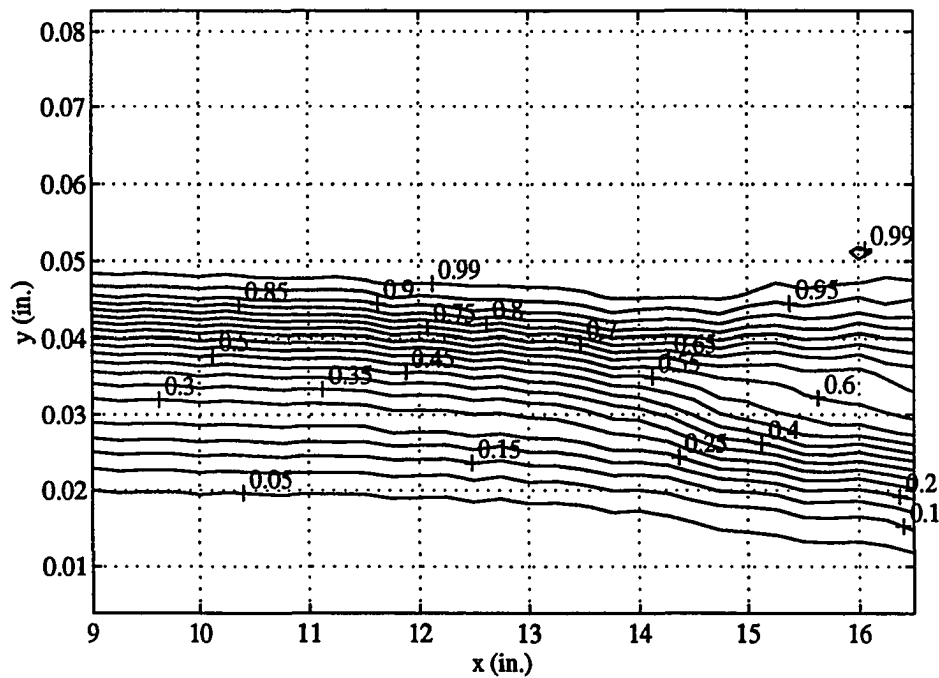
Figure 4.4 Contour Plot of Normalized V_{s,mean} (Adiabatic Cone)
