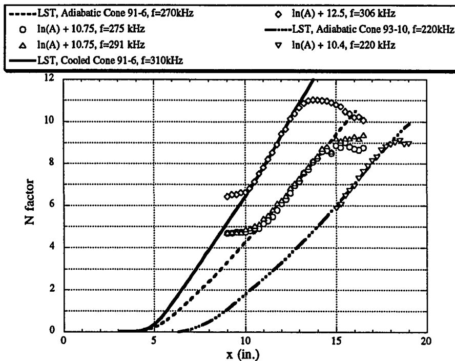
Figure 7.3 Growth Plot for all Experimental Data
