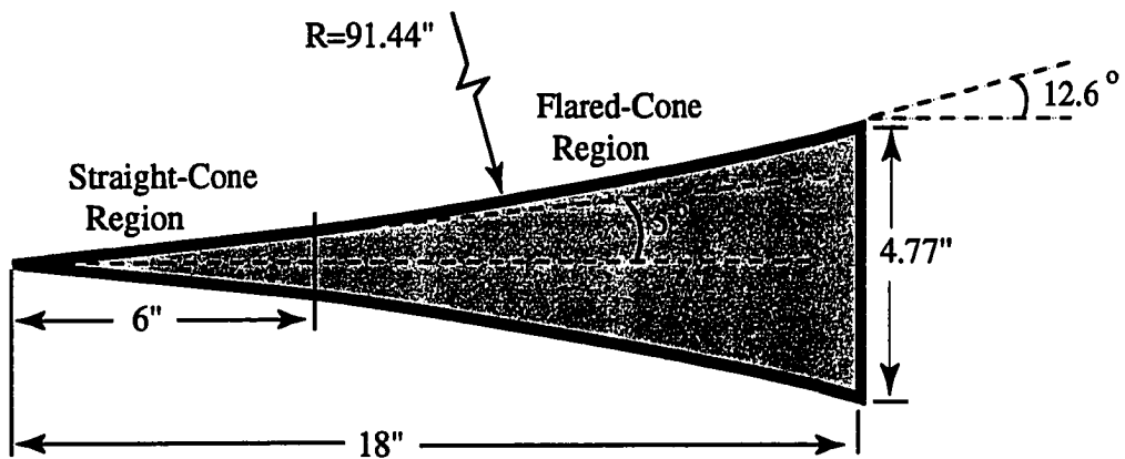
Figure 1.2 Geometry of the 91-6 Cooled-Cone Model
