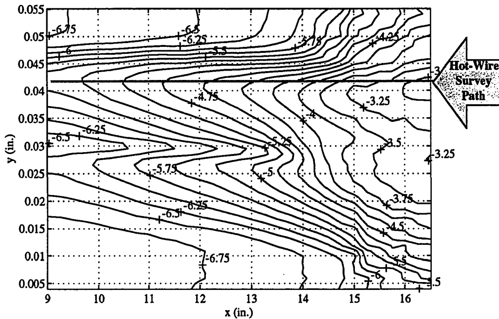
Figure 4.8 Hot-Wire Survey Path and RMS Contours (Adiabatic Cone)
