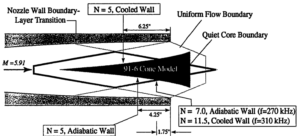
Figure 2.3 Cone 91-6 in M6NTC with Quiet Core
