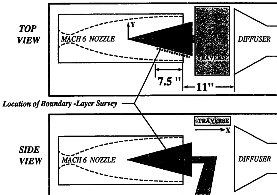
Figure 2.7 Traversing Line over Cone and Coordinate System
