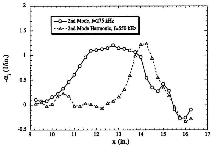
Figure 4.15 Second-Mode and Harmonic Growth Rates (Adiabatic Cone)
