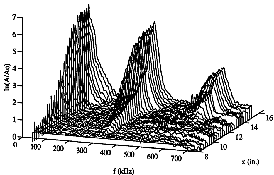
Figure 4.9 Disturbance Spectra in the Adiabatic-Cone Boundary Layer (Oblique View)
