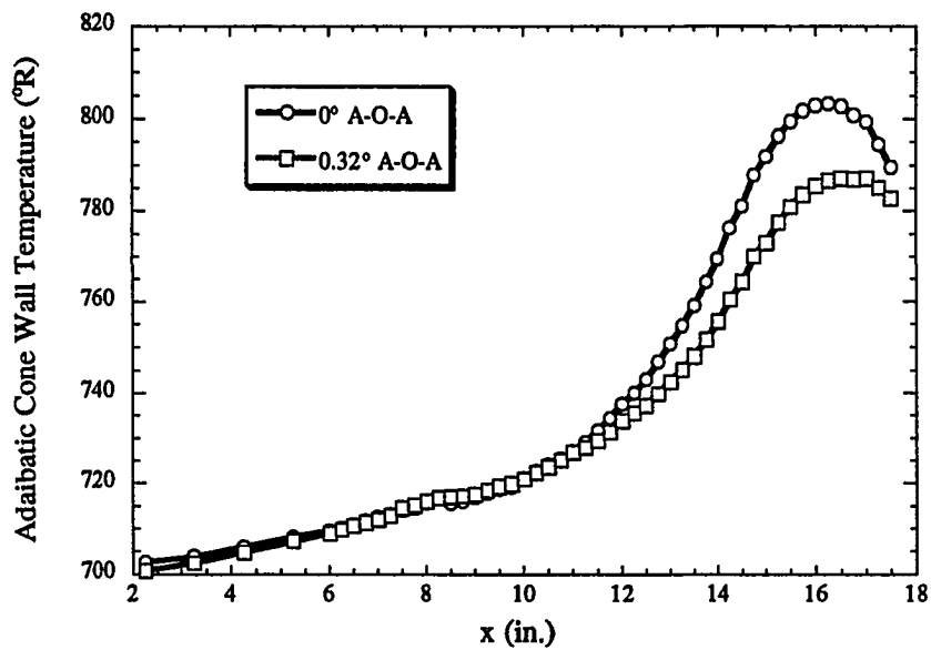
Figure 6.8 Variation in Wall Temperature with A-O-A (Windward Side Measurements)
