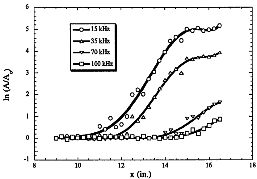
Figure 4.16 Low-Frequency Disturbances in the Adiabatic-Cone Boundary Layer
