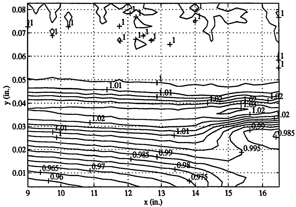
Figure 4.3 Contour Plot of Normalized R_w (Adiabatic Cone)
