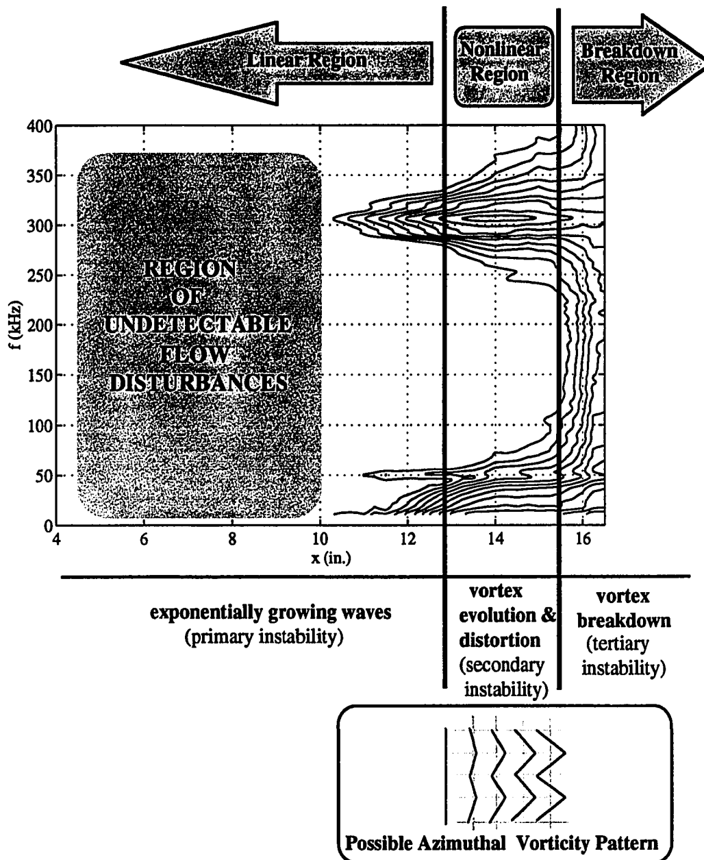
Figure 7.1 Identifiable Flow Regions for a Hypersonic Flow Undergoing Transition (Contour Plot of Cooled Cone data previously presented in Fig. 5.11)
