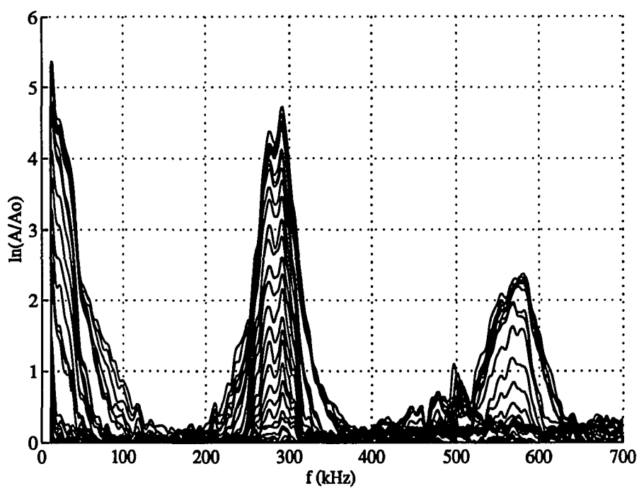
Figure 4.10 Disturbance Spectra in the Adiabatic-Cone Boundary Layer (Front View)
