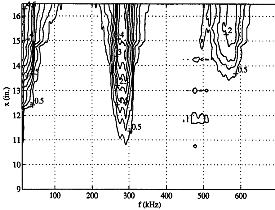
Figure 4.11 Disturbance Spectra in the Adiabatic-Cone Boundary Layer (contour plot) (contours based on \ln(A/A_0) data in 0.5 increments from 0.5)
