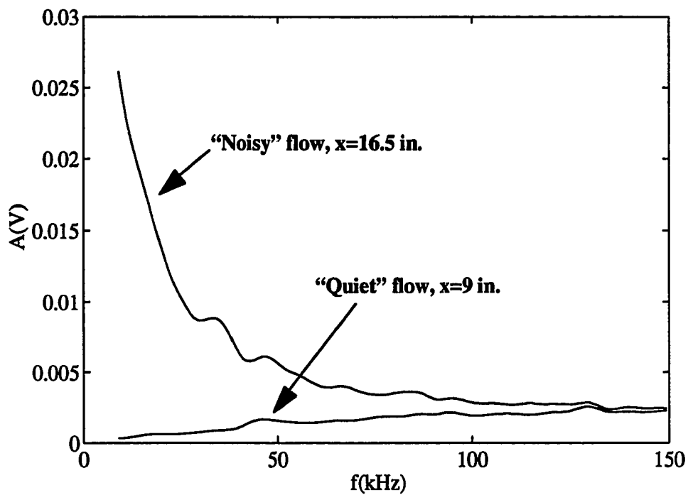
Figure 3.1 "Quiet" and "Noisy" Flow at y = 0.24 in.
