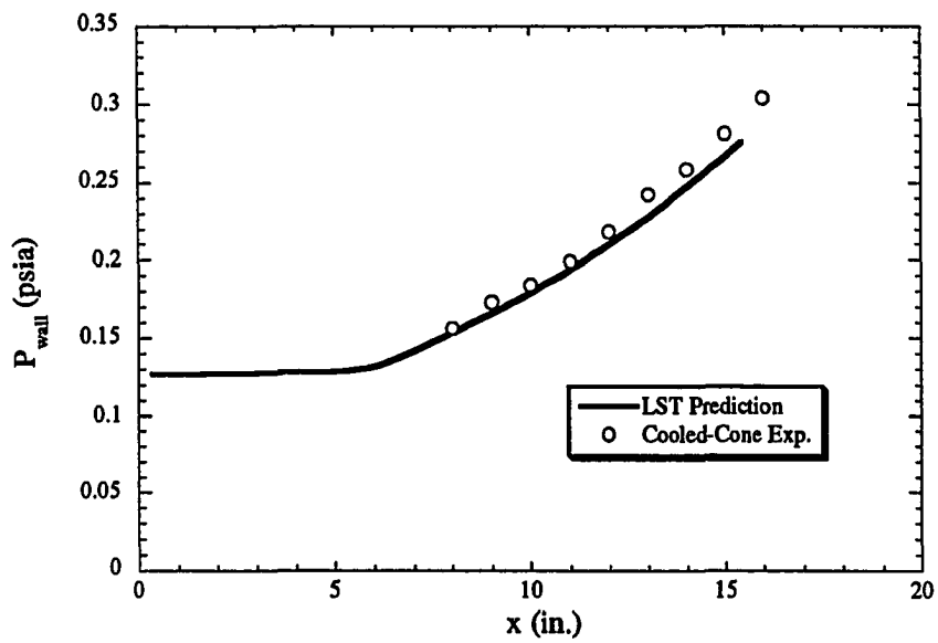
Figure 5.6 Wall Static Pressure (Cooled Cone)
