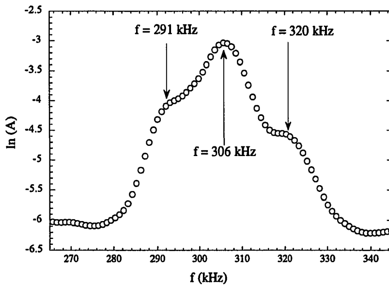
Figure 5.12 Second-Mode Disturbance Band (Cooled Cone, x=12 in.)
