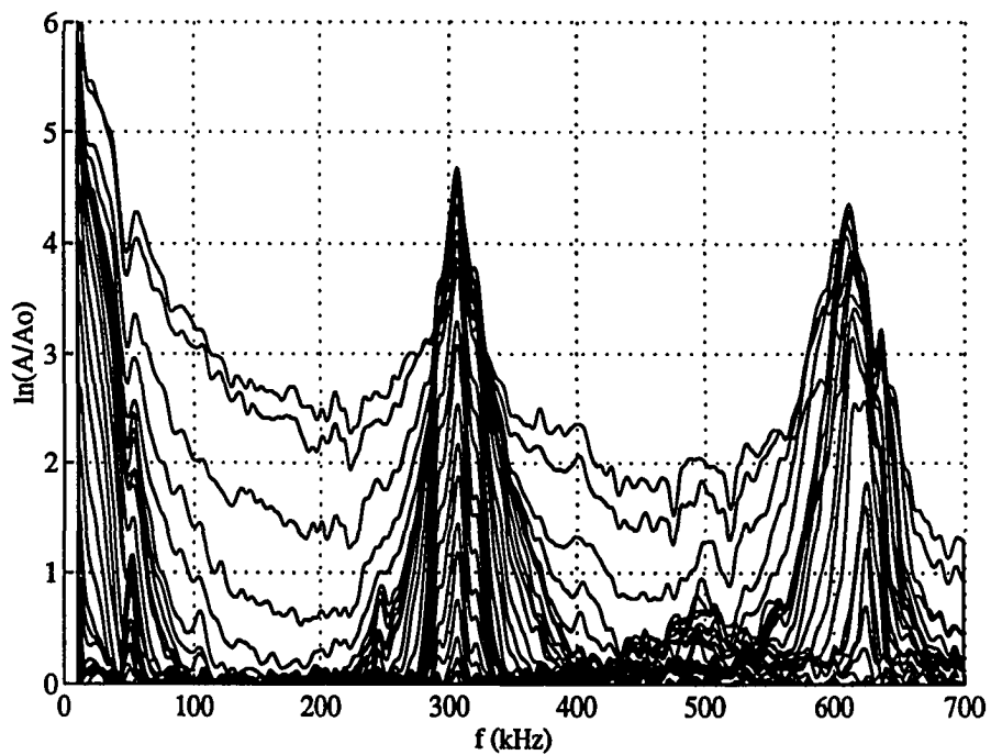
Figure 5.10 Disturbance Spectra in the Cooled-Cone Boundary Layer (Front View)
