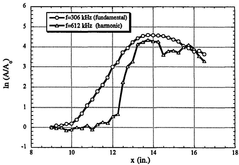
Figure 5.15 Growth of Second-Mode Disturbance and Harmonic (Cooled Cone)
