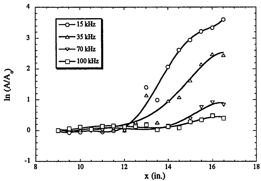
Figure 3.4 Low-Frequency Disturbances in the Freestream
