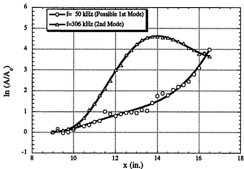
Figure 5.17 Growth of the Second Mode and a Possible First Mode (Cooled Cone)
