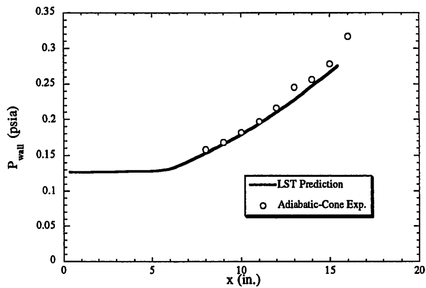
Figure 4.6 Wall Static Pressure (Adiabatic Cone)
