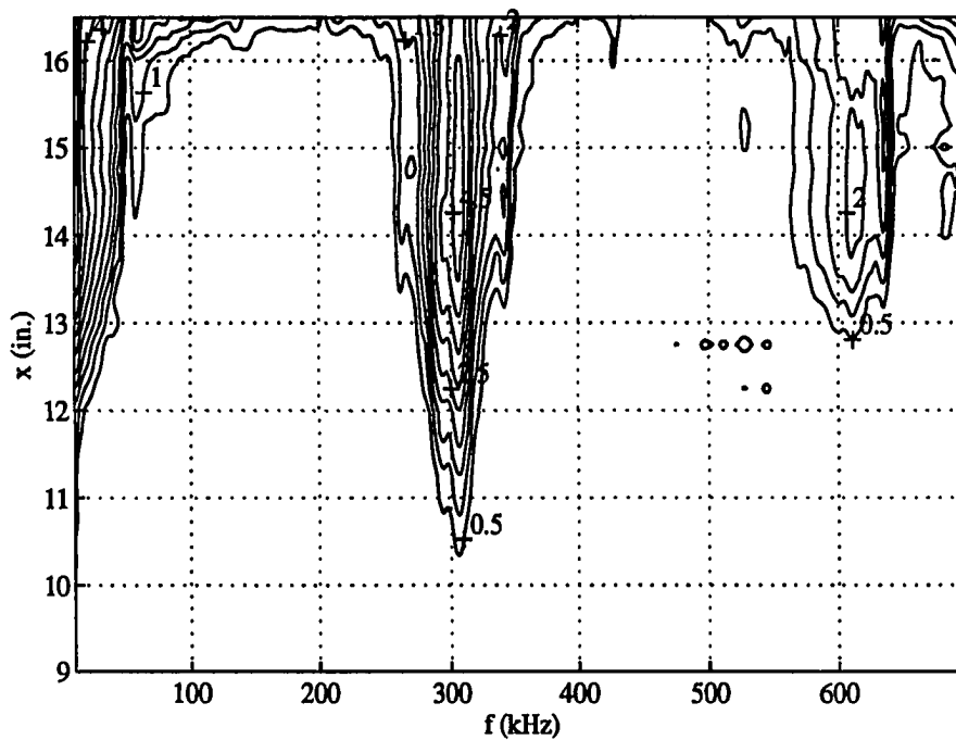
Figure 6.6 Disturbance Spectra in the Minimally-Cooled Boundary Layer
