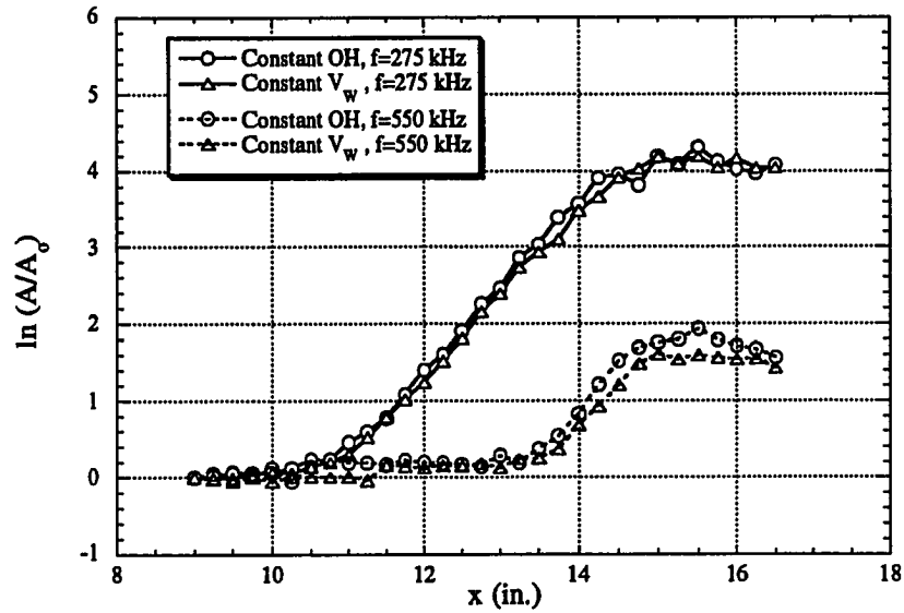
Figure 6.1 Sensitivity of CVA Operation Mode to Adiabatic-Cone Disturbances
