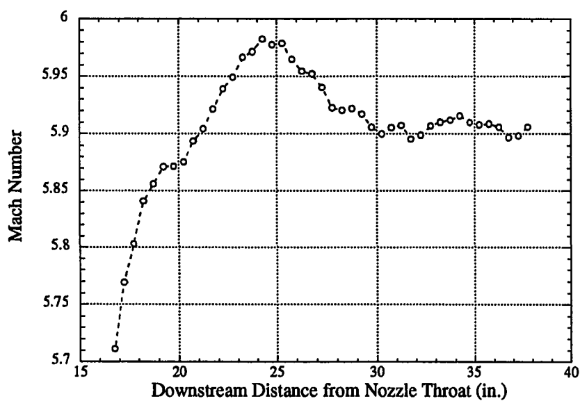
Figure 2.2 Centerline Mach Number of the M6NTC at Re_\infty = 2.85 \times 10^6 / \text{ft} .
