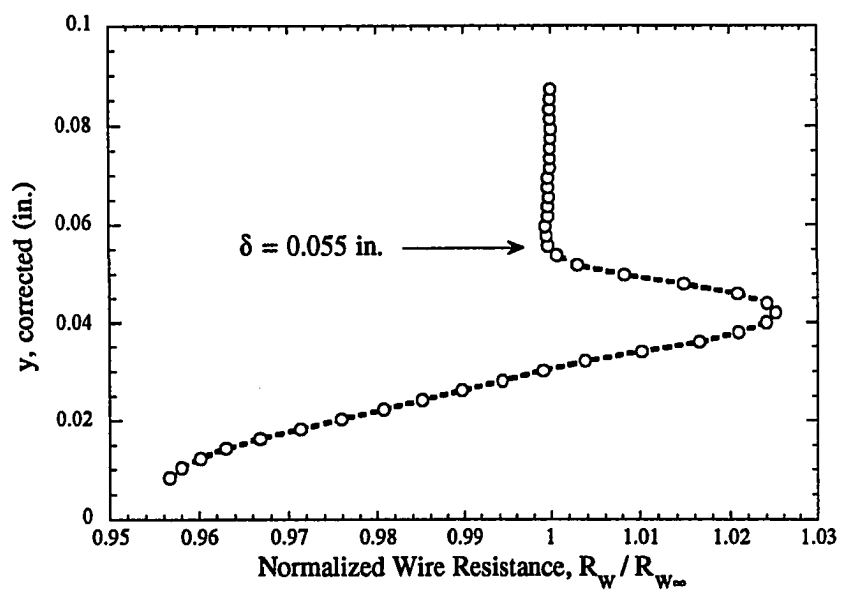
Figure 4.2 Resistance of Unheated Hot Wire at x=9.00 in. (Adiabatic Cone)
