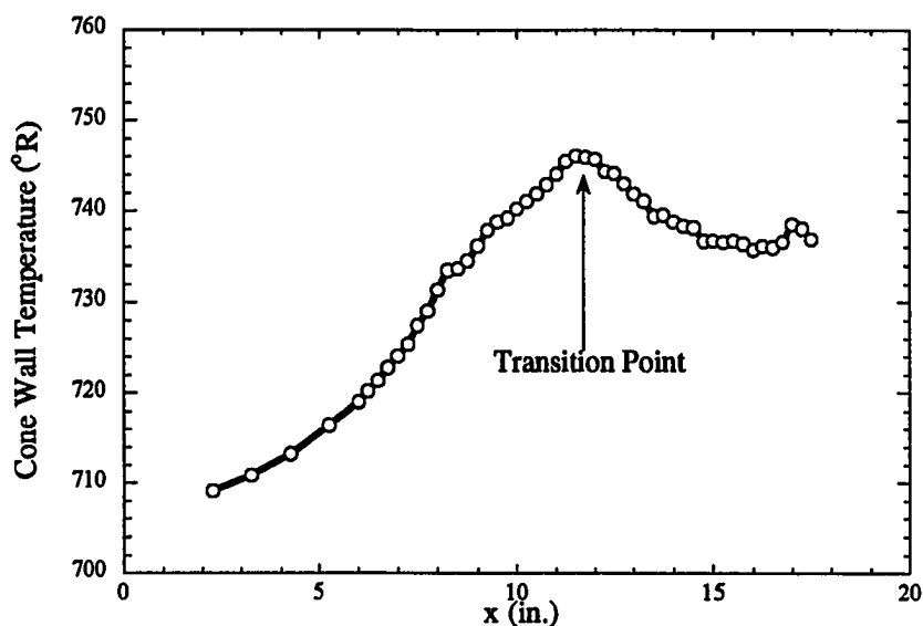
Figure 7.2 Wall Temperature of the Adiabatic Cone with High Noise Level
