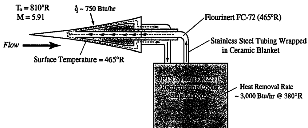
Figure 2.1 Active Cooling System for the Cooled Cone
