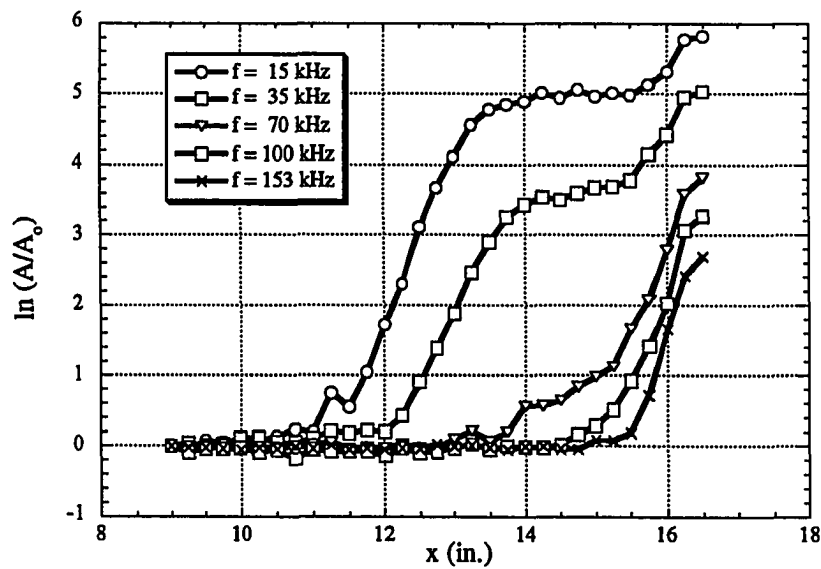
Figure 5.16 Low-Frequency Disturbances in the Cooled-Cone Boundary Layer
