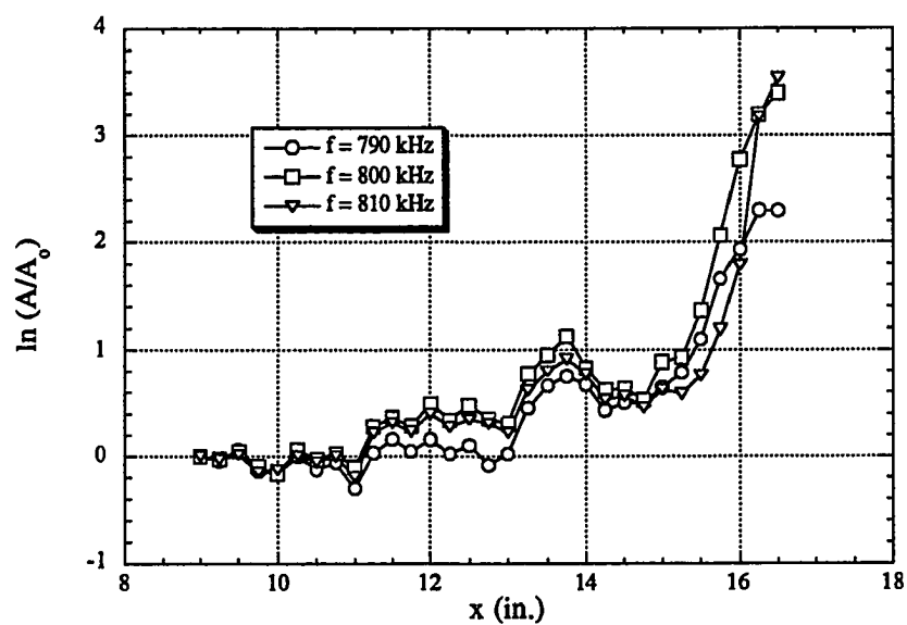
Figure 5.19 Growth of the Unknown Disturbance Band Identified in Fig. 5.18
