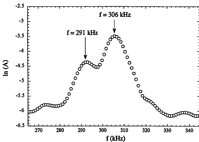
Figure 6.4 Second-Mode Disturbance Band (Minimum Cooling, x=12 in.)
