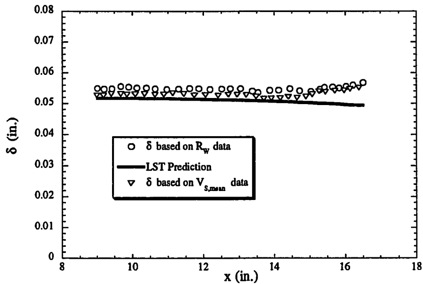
Figure 4.5 Boundary-Layer Thickness (Adiabatic Cone)
