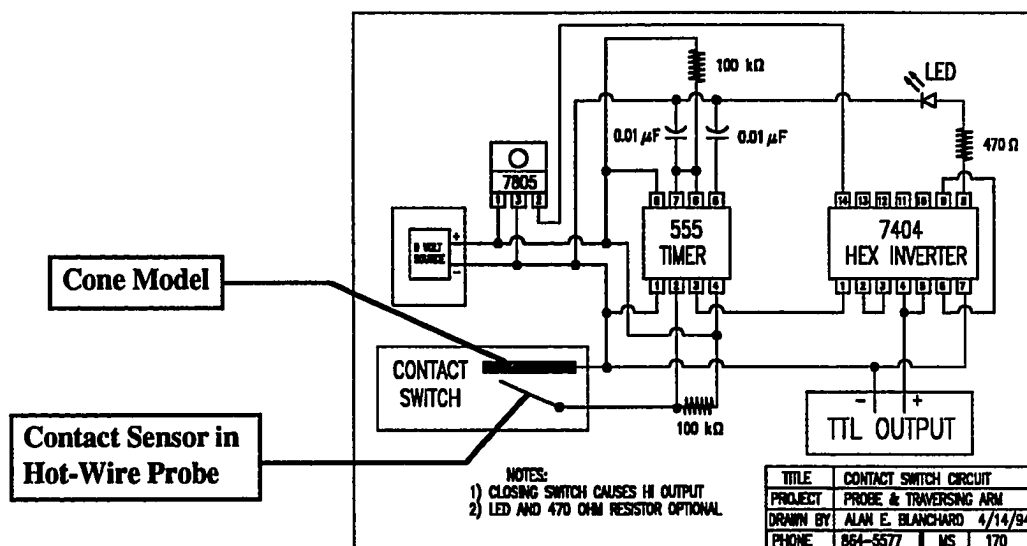
Figure 2.5 Contact Circuit Schematic
