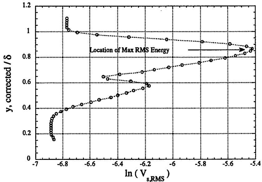
Figure 4.7 RMS Energy at x=9.00 in. (Adiabatic-Cone)
