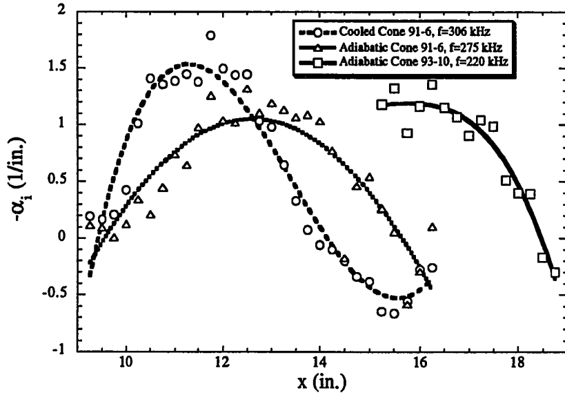
Figure 7.4 Dimensional Growth Rates from Fig. 7.3
