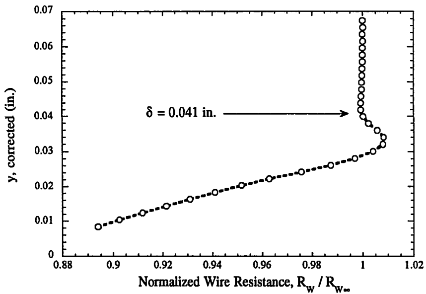
Figure 5.2 Resistance of Unheated Hot Wire at x=9.00 in. (Cooled Cone)
