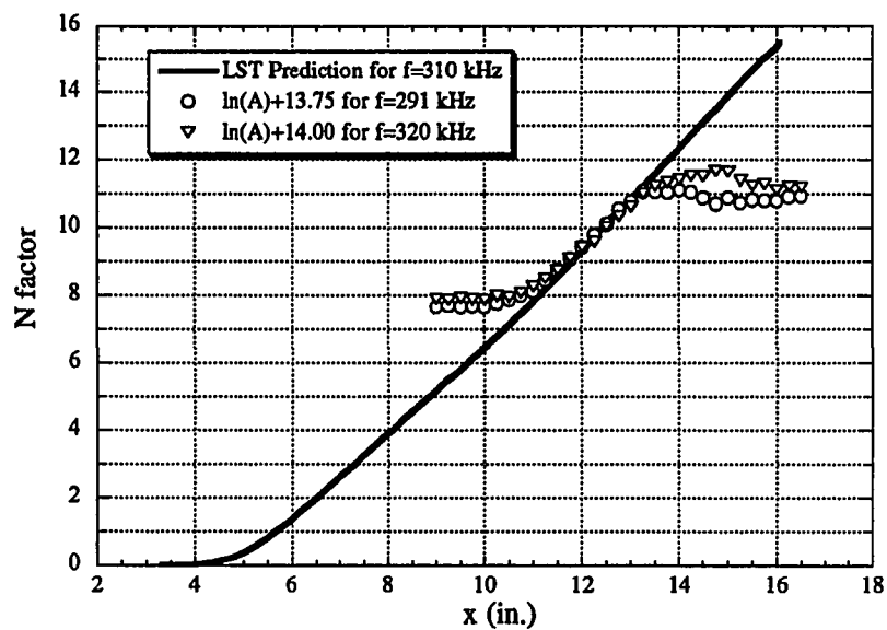
Figure 5.14 Growth Chart for 291 and 320 kHz (Cooled Cone)
