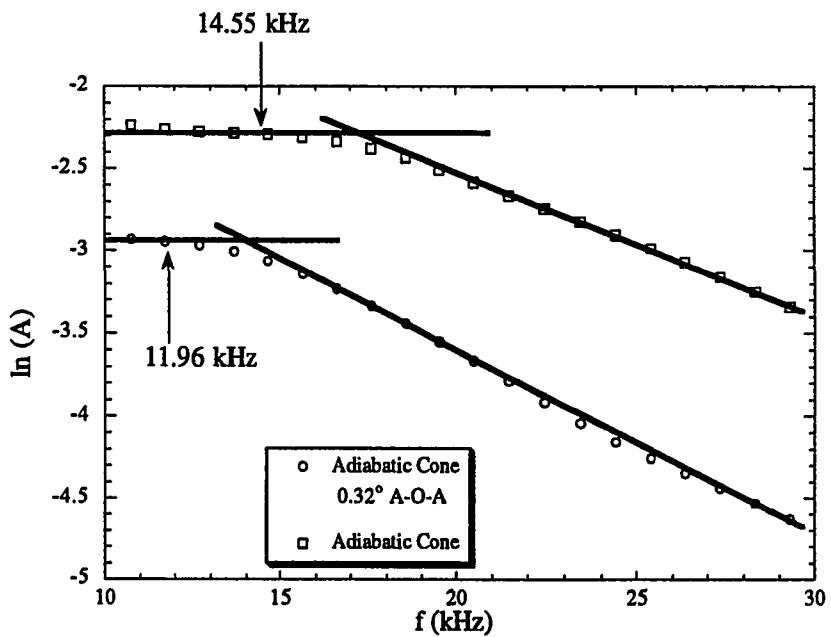
Figure 7.5 Low-Frequency Data Associated with Fig. 6.10 Spectra
