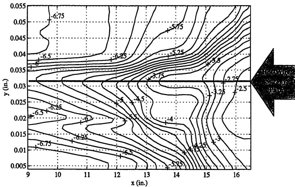
Figure 5.8 Hot-Wire Survey Path and RMS Contours (Cooled Cone)
