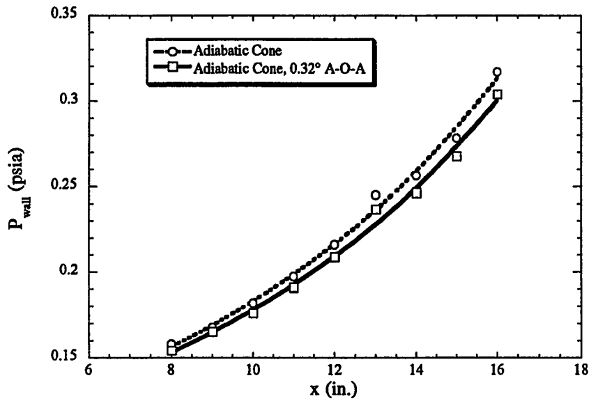
Figure 6.7 Variation in Wall Pressure with A-O-A (Leeward Side Measurements)
