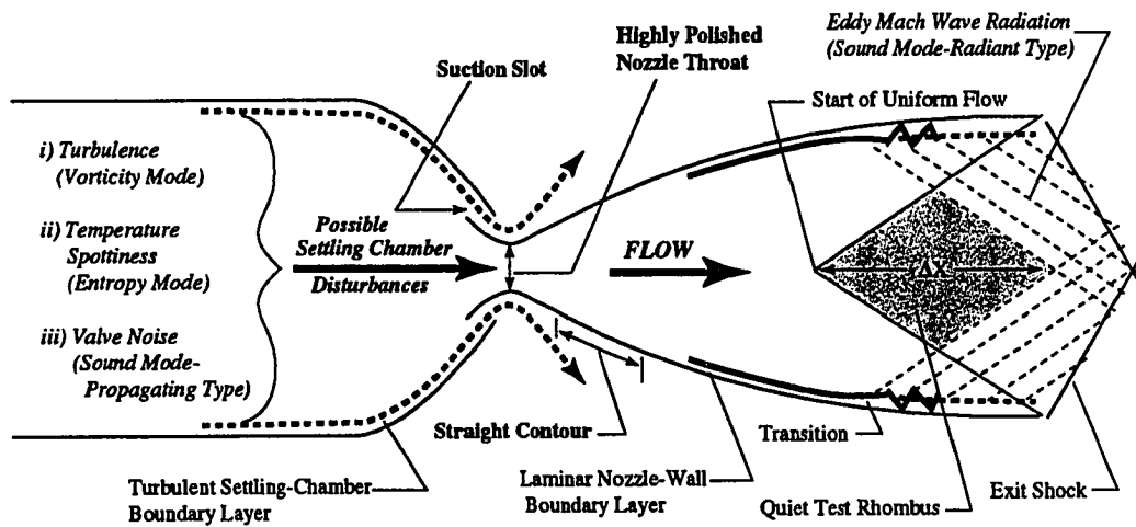
Figure 1.3 Typical Quiet Tunnel
