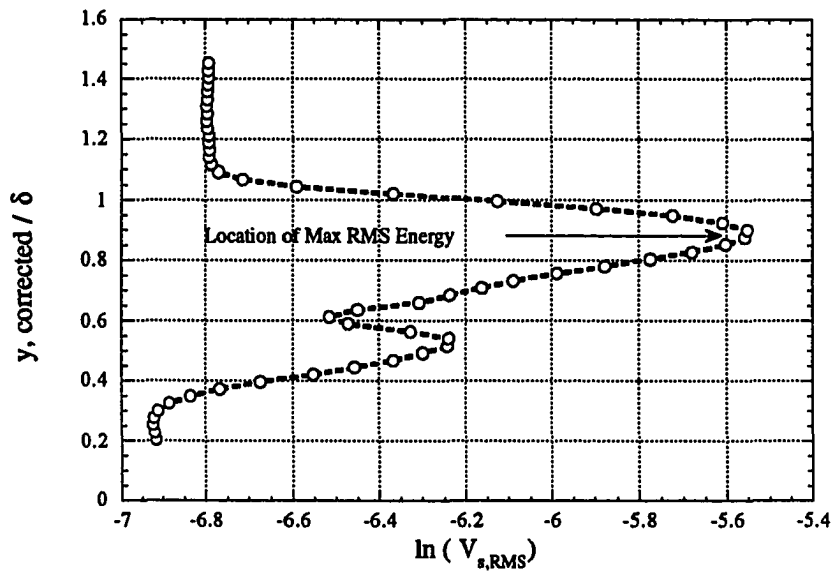
Figure 5.7 RMS Energy at x=9.00 in. (Cooled Cone)
