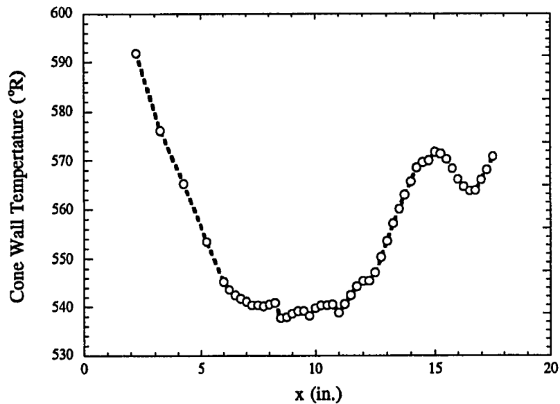
Figure 6.2 Wall Temperature of the Cone with Minimum Cooling
