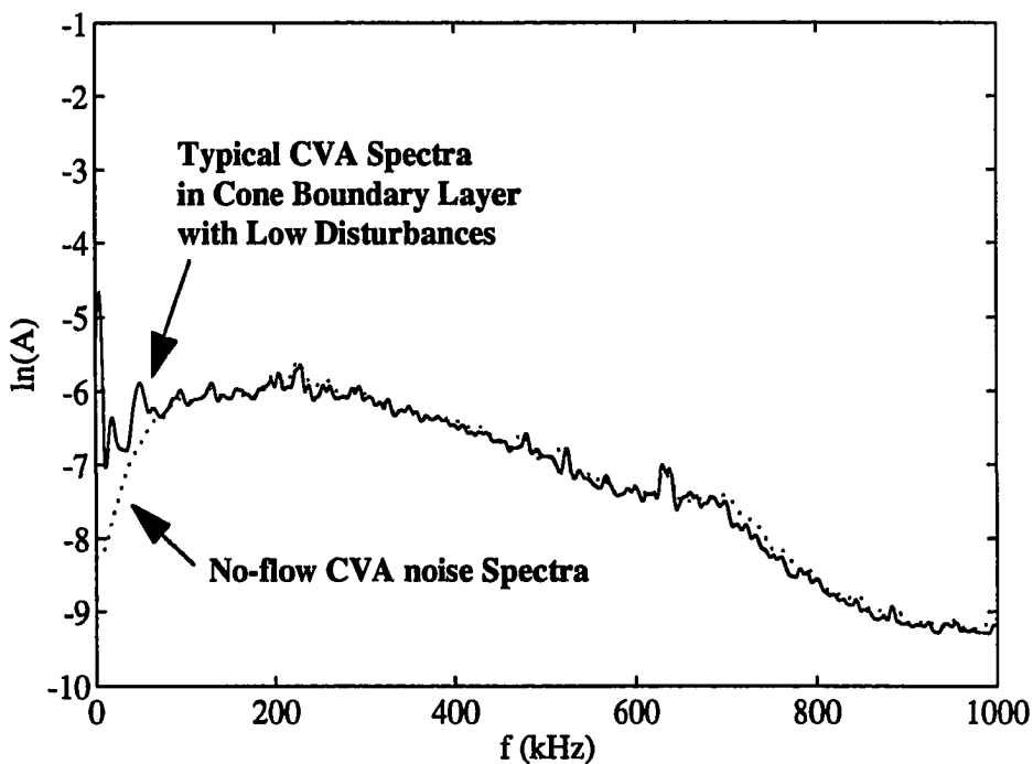
Figure 2.6 CVA Noise Spectra and Hot-Wire Low-Disturbance Spectra
